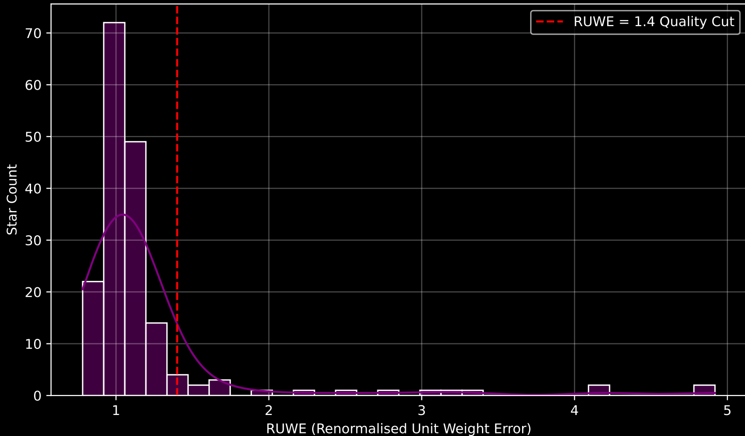
GAPOGEE DR17 Field [288-35-O_TESS] RUWE Distribution (n= 177)
