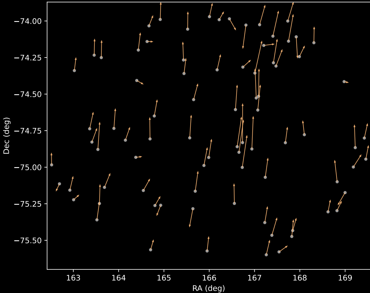
APOGEE DR17 Cluster 3 Proper Motion Vectors (n=82)
