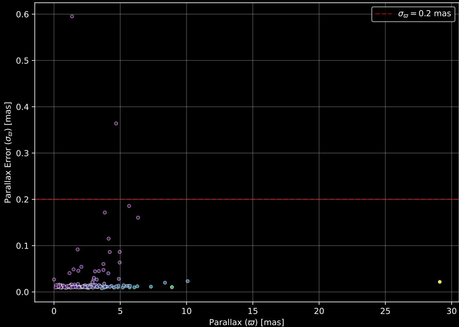
APOGEE DR17 Field: [288-35-O_TESS] Parallax Quality (n= 188)
