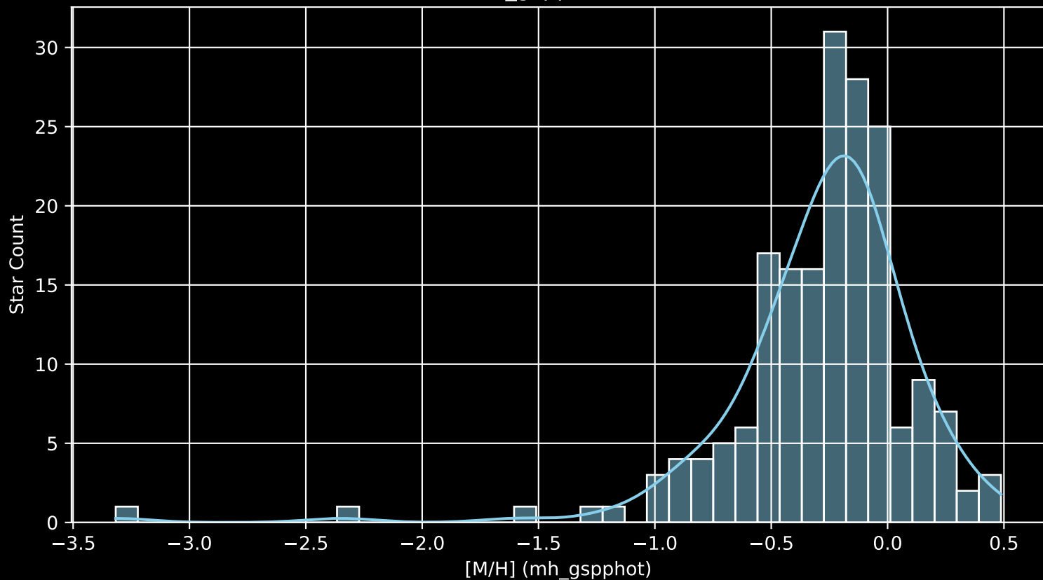
APOGEE DR17 Field: [288-35-O_TESS [M/H] (mh_gspphot) (n= 187)
