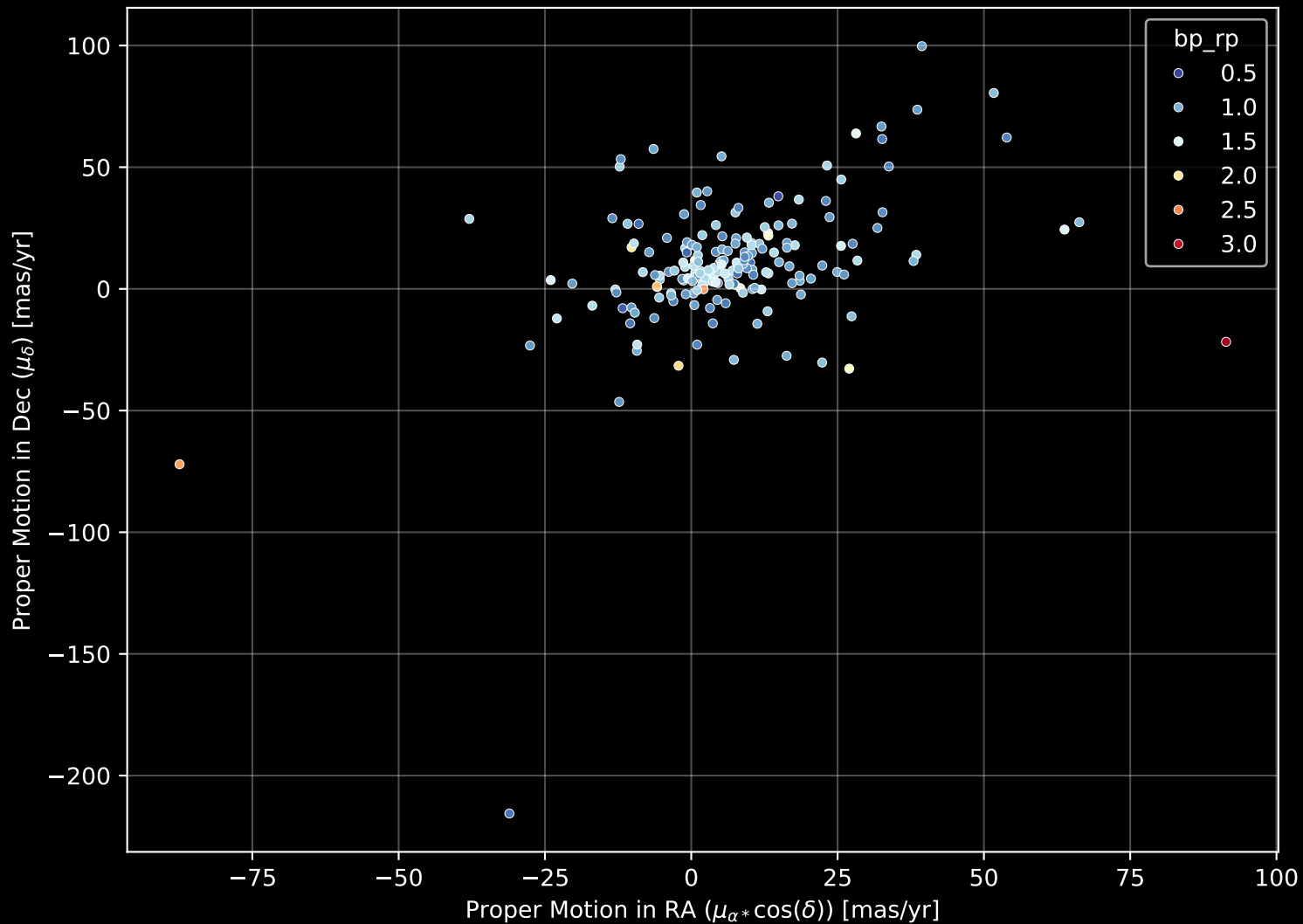
APOGEE DR17 Field: [288-35-O_TESS] Proper Motion Diagram (n= 188)
