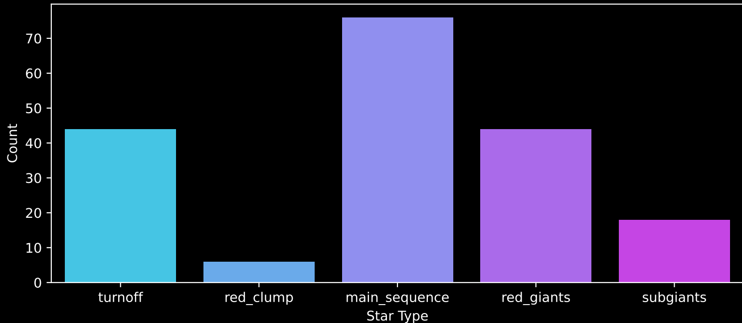
APOGEE DR17 Field: [288-35-O_TESS] Count plot of Star Type
